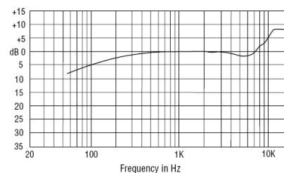
Frequency Response
